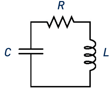
Figure 3: Circuit equivalent of an electromagnetic resonator
